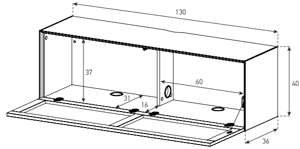
ED 61-TS (WITH CABLE MANAGEMENT)
