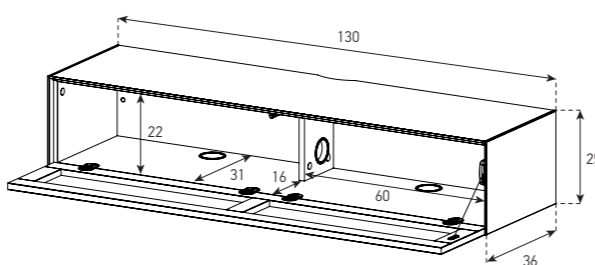
ED 66-TS (WITH CABLE MANAGEMENT)
