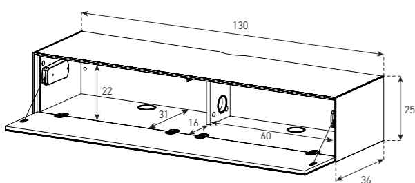
ED 66-F (WITH CABLE MANAGEMENT)
